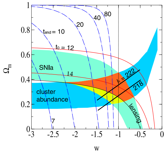
FIG. 2: Same as in Fig. 1, except extended to w < -1 . Here, the blue dot-dash curves show for phantom-energy ( w < -1 ) models the time (in Gyr) remaining in the Universe (assuming a Hubble parameter H_0 = 70 \text{ km sec}^{-1} \text{ Mpc}^{-1} ).
