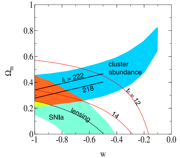
FIG. 1: Current constraints to the w - \Omega_m parameter space. The red solid curves show the age (in Gyr) of the Universe today (assuming a Hubble parameter H_0 = 70 \text{ km sec}^{-1} \text{ Mpc}^{-1} ). The light shaded regions are those allowed (at 2\sigma ) by the observed cluster abundance and by current supernova measurements of the expansion history. The dark orange shaded region shows the intersection of the cluster-abundance and supernova curves, additionally restricted (at 2\sigma ) by the location of the first acoustic peak in the cosmic-microwave-background power spectrum and quasar-lensing statistics.
